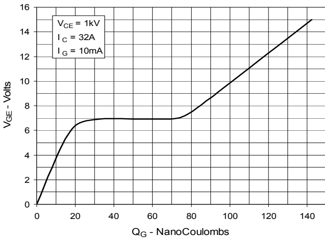
Fig. 9. Gate Charge
