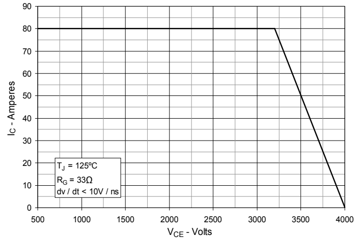
Fig. 6. Reverse-Bias Safe Operating Area
