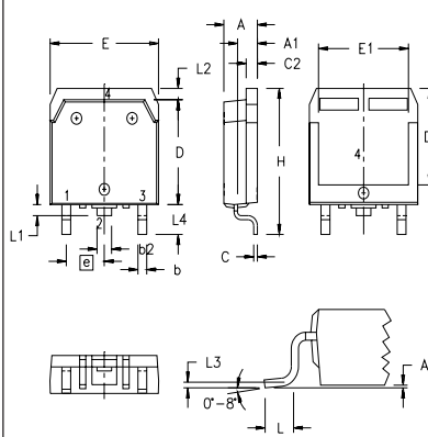
TO-268 (IXFT) Outline
