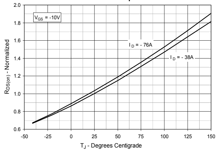
Fig. 4. R_{DS(on)} Normalized to I_D = -38\text{A} vs. Junction Temperature
