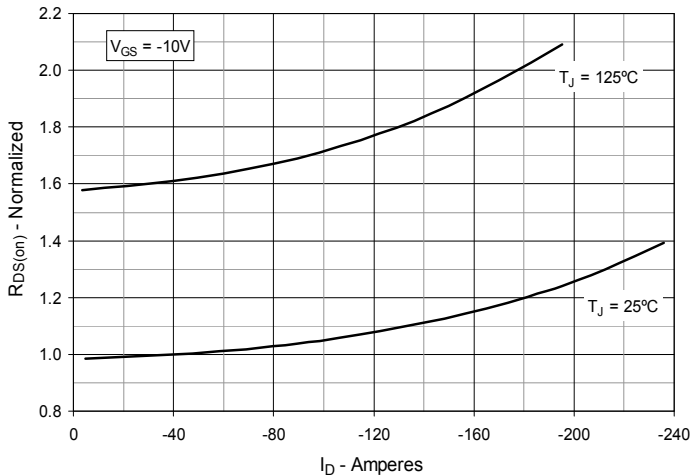
Fig. 5. R_{DS(on)} Normalized to I_D = -38\text{A} vs. Drain Current
