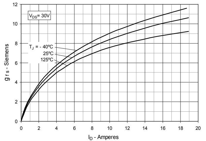
Fig. 10. Transconductance
