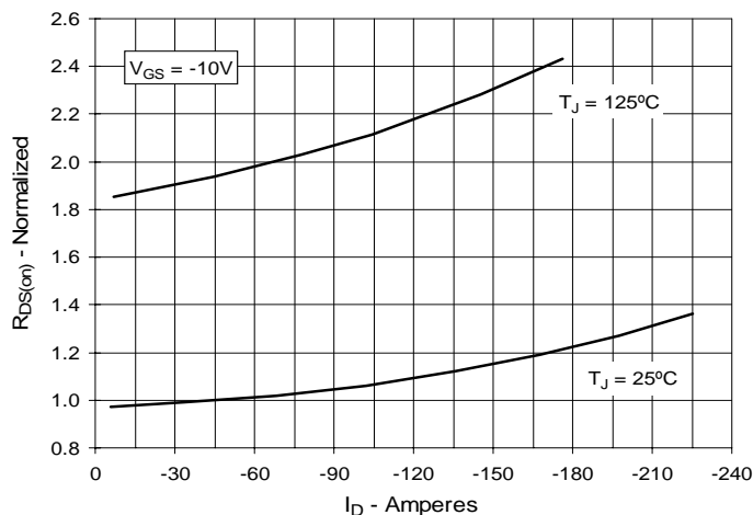
Fig. 5. R_{DS(on)} Normalized to I_D = -45A . Drain Current
