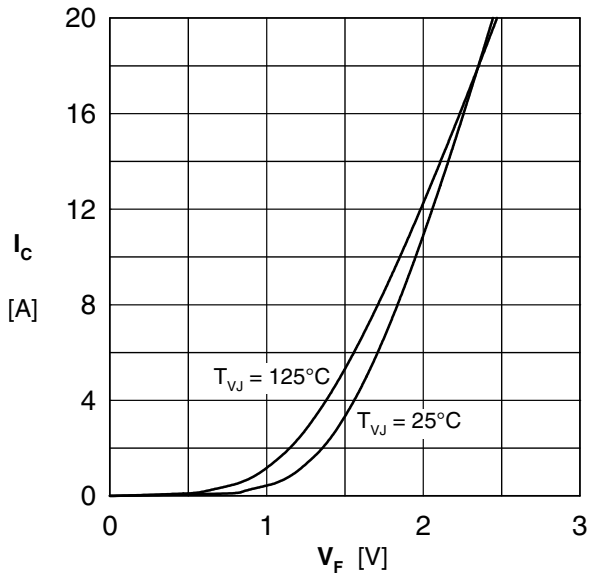
Fig. 7 Typ. forward characteristic
